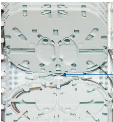
▲ Langmatz organiser and fibre trays
