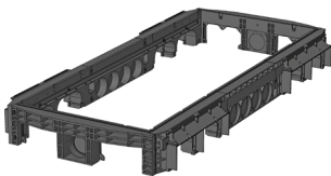
Frame 220 mm overbuild Art. no.: 06 738 0087E 2 x rectangular / 1 x Ø 110 4 x rectangular / 4 x Ø 110 Weight: 72.5 kg
