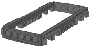
Frame 220 mm overbuild Art. no.: 06 738 0085E 5 x Ø 110 4 x rectangular / 4 x Ø 110 Weight: 73.0 kg
