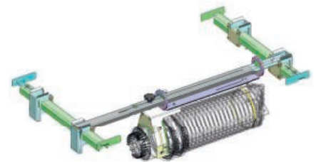
Swivelling arm/Pivoting telescopic fibre closure bracket Attachment to the crossbar
