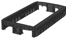
Frame 220 mm Art. no.: 06 708 0061E 2 x rectangular / 1 x Ø 110 8 x Ø 110 Weight: 49.0 kg
