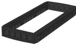
Frame 220 mm Art. no.: 06 748 0052E 5 x Ø 110 12 x Ø 110 Weight: 67.0 kg
