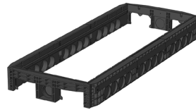
Frame 220 mm Art. no.: 06 748 0061E 2 x rectangular / 1 x Ø 110 12 x Ø 110 Weight: 61.5 kg
