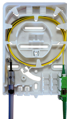
Example: use as termination box (STB)
