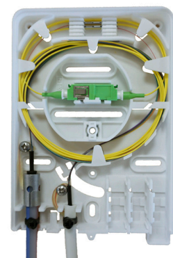
Example: use as indoor / outdoor connection point (OFD)
