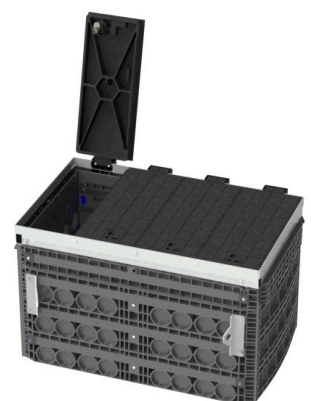
Rectangular hinged cover EK 428 on an example manhole; 1 cover opened
